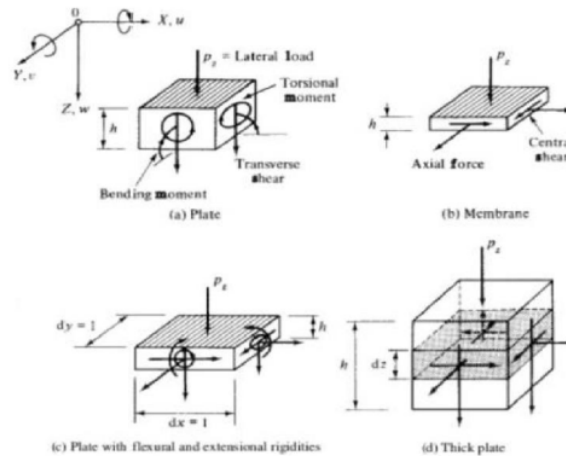
Figure 1. Inner Forces on Different Types of Plates
